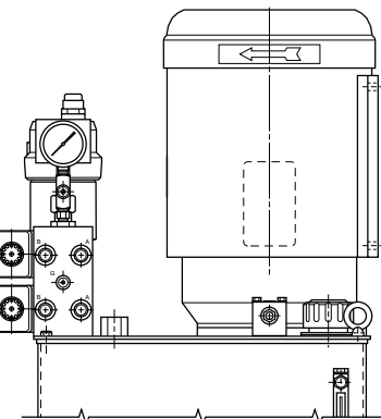
"M5" OPTION MANIFOLD (MULTI-STATION D05 MANIFOLD) SHOWN WITH OPTION "N" RETURN FILTER
